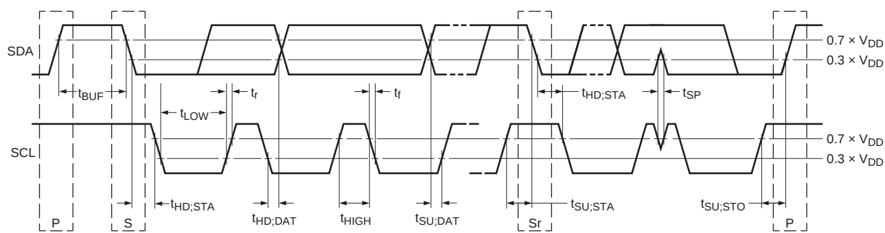
Fig 19. Definition of timing
