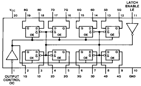
Top View MM74HCT373
