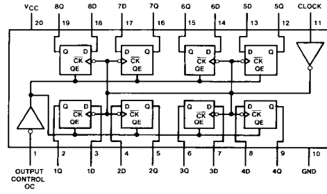
Top View MM74HCT374
