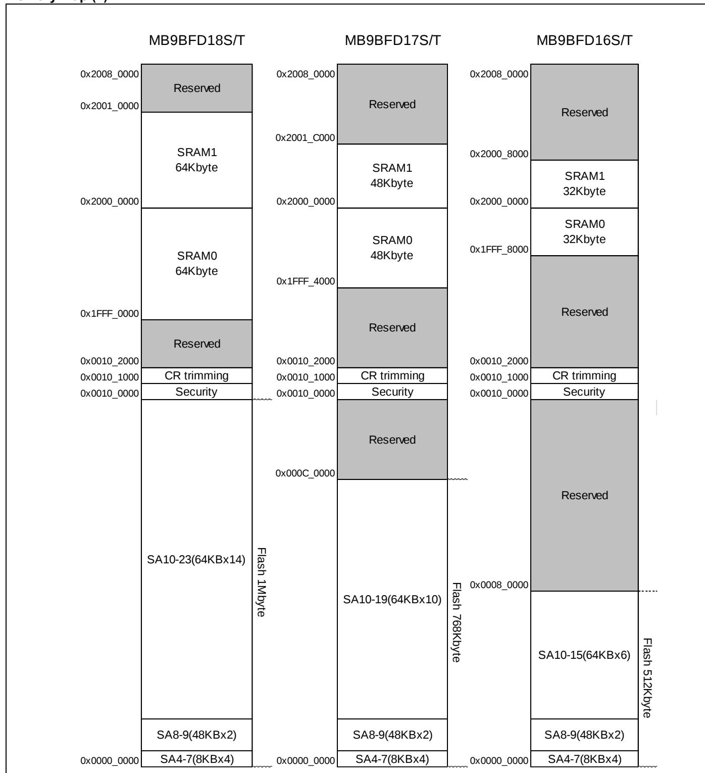
Memory Map (2)
