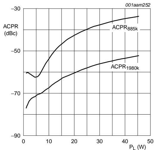
Fig 5. Single carrier IS-95 ACPR at 885 kHz and at 1980 kHz as function of load power; typical values
