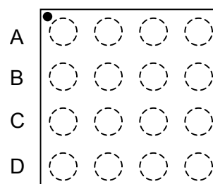
16-Ball CSBGA (4mm x 4mm)
