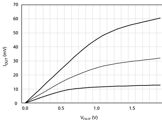
Figure 18: Reduced Strength Pull-Down Characteristics
