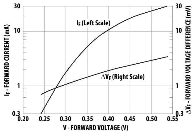
Figure 2. Typical VF Match, HSMS-820X Pairs and Quads.
