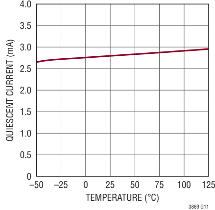
Quiescent Current without EXT CC vs Temperature
