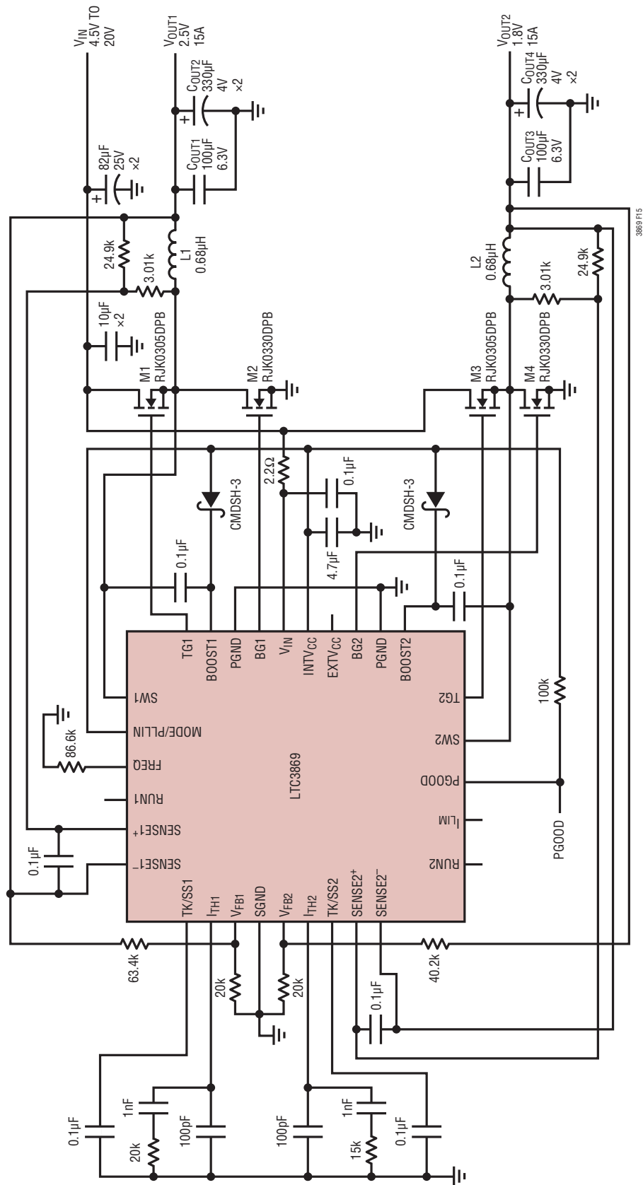
L1, L2: VISHAY IHL5050CE-01, 0.68 \mu H COUT1: MURATA GRM32ER60J107ME20 COUT2: COUT3: KEMET T520V337M004ATE009 RNTC1, RNTC2: MURATA NCP18WF104J03RB
