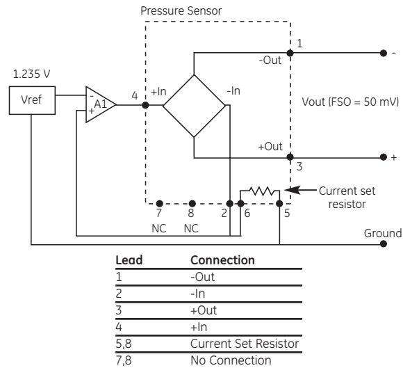
NPC-1220 Series schematic Diagram
