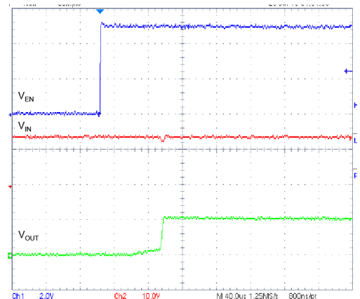
Figure 37. Enable transient ( I_{OUT} = 400\text{ mA} )
