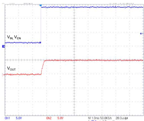
Figure 38. Start-up transient ( I_{OUT} = 0.1\text{ mA} )
