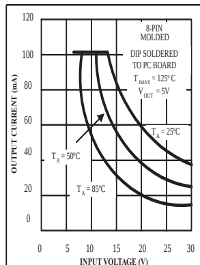
LP2950 Maxium Rated Output Current
