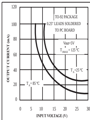
LP2950 Maxium Rated Output
