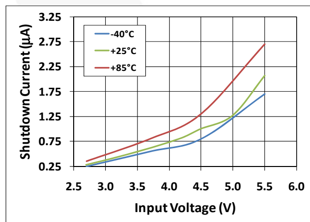
Figure 15. Shutdown Current vs. Input Voltage vs. Temperature
