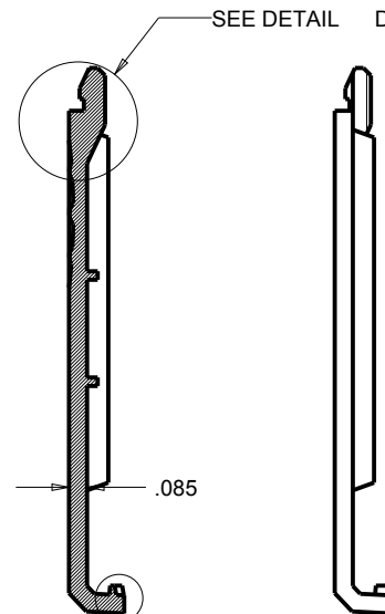
SECTION X-X
