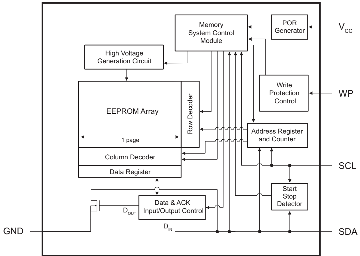
Figure 2-1. Block Diagram
