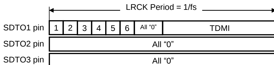
Figure 57. Slot Assign in PCM Mode
