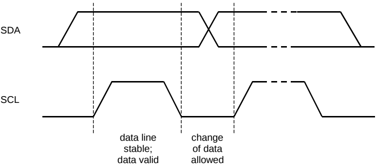
Figure 71. Bit Transfer on the I 2 C-Bus
