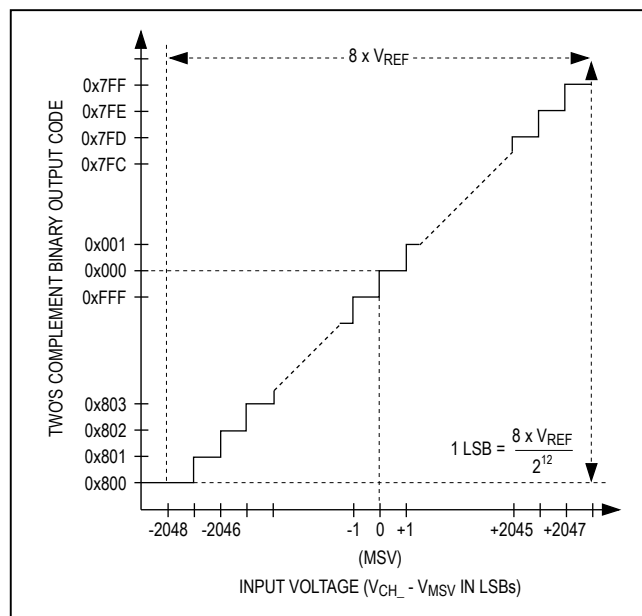
Figure 14. \pm 10\text{V} Bipolar Transfer Function
