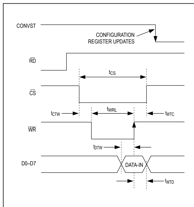
Figure 6. Write Timing
