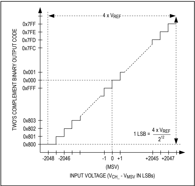
Figure 13. \pm 5\text{V} Bipolar Transfer Function
