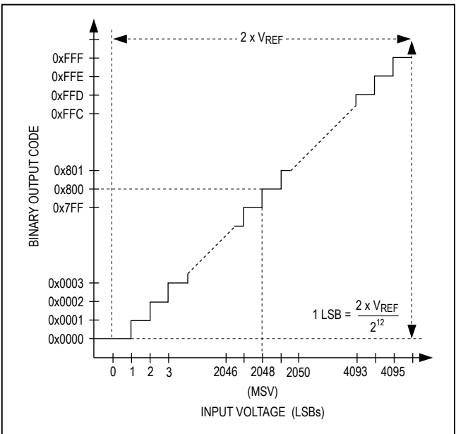
Figure 12. 0 to +5V Unipolar Transfer Function
