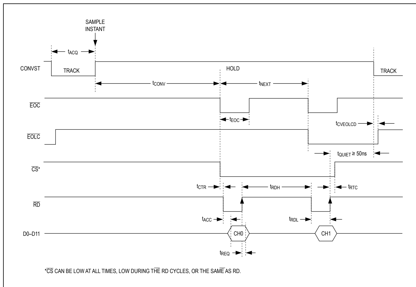
Figure 7. Read During Conversion—Channel 0 and Channel 1 Selected, Internal Clock
