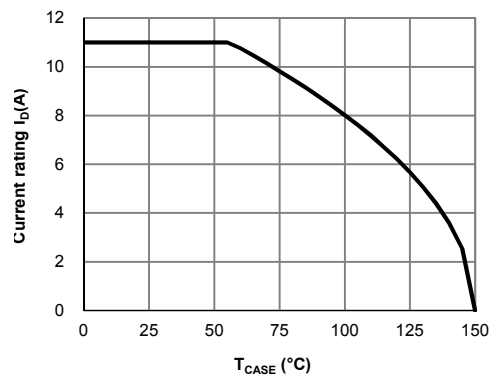
Figure 12: Current De-rating (Note B)
