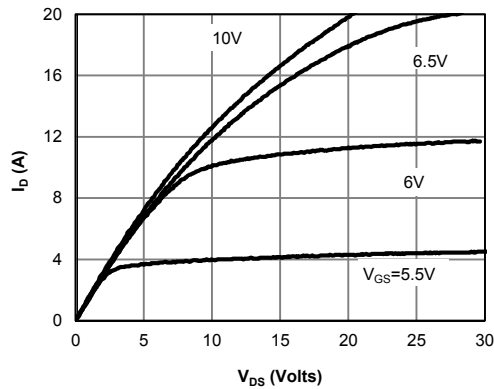
Fig 1: On-Region Characteristics
