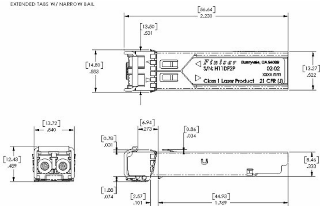
FWLF15217Dxx Outline Drawing - units in inches [mm]
