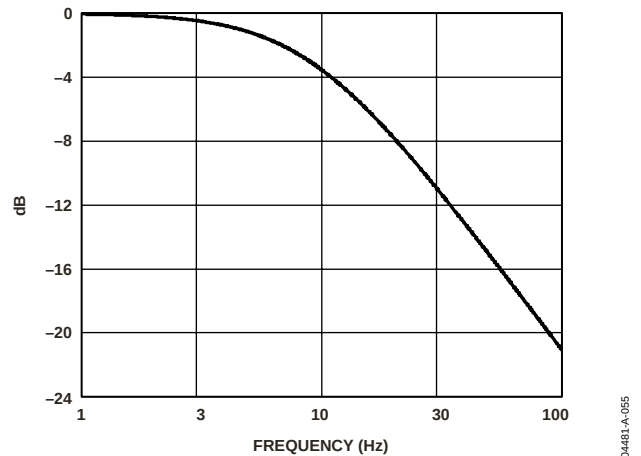
Figure 54. Frequency Response of LPF2
