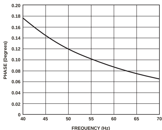
Figure 51. Combined Phase Response of HPF and Phase Compensation (40 Hz to 70 Hz)
