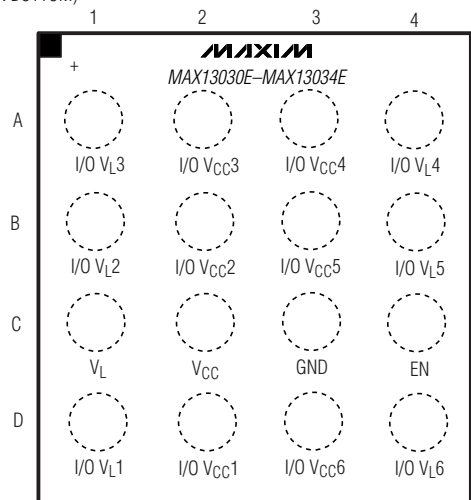
16 UCSP (2mm x 2mm)
