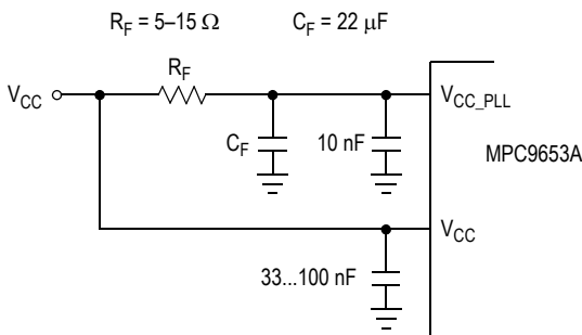
Figure 3. \text{V}_{\text{CC\_PLL}} Power Supply Filter
