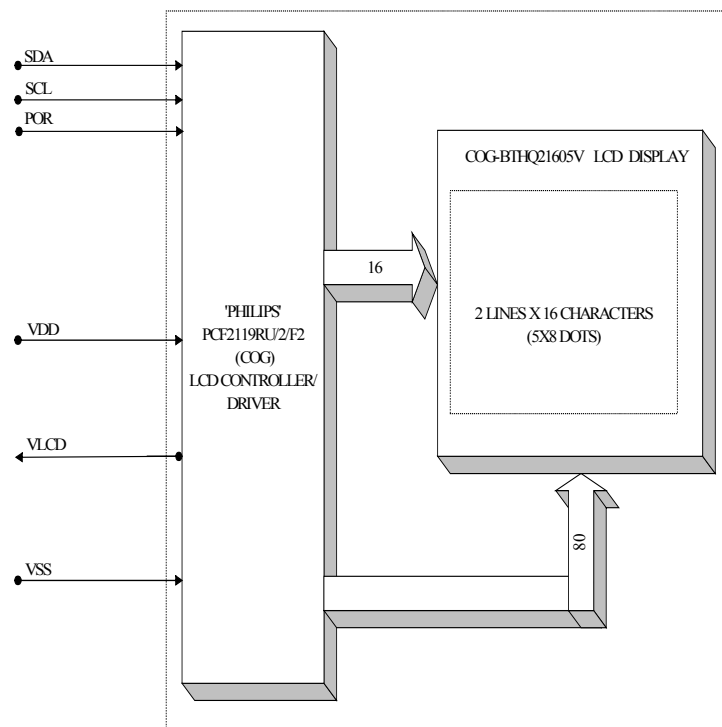
Figure 4: Block Diagram
