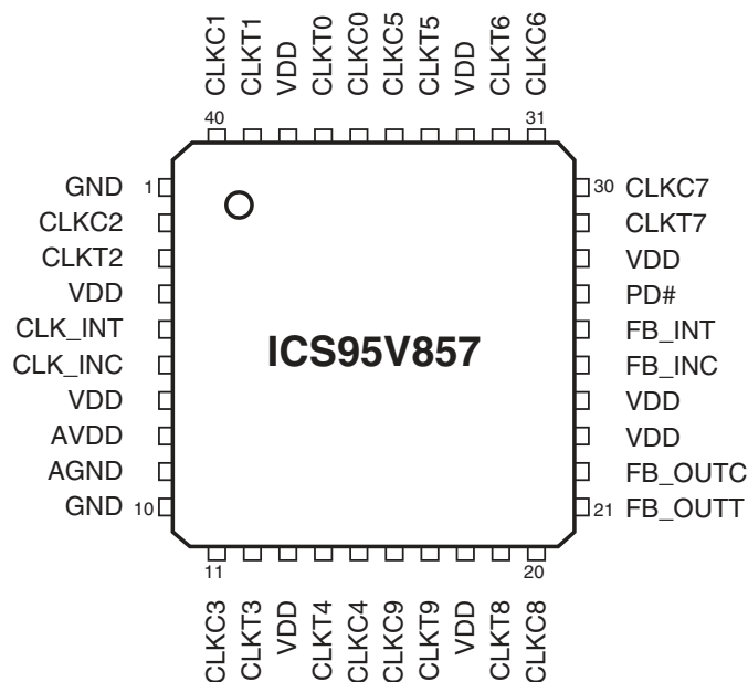
40-Pin MUF
