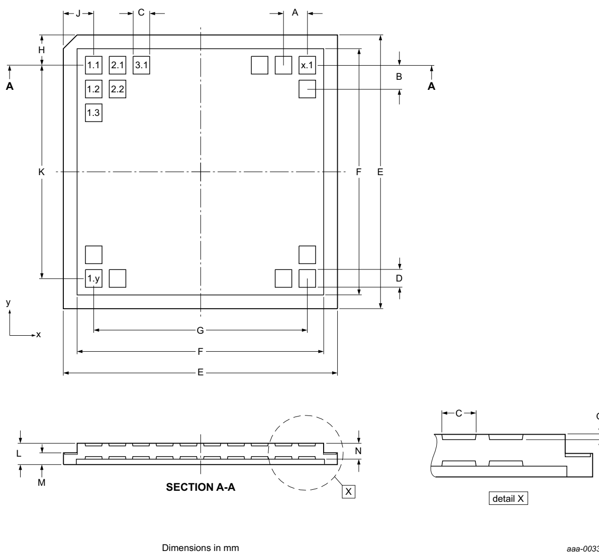
Fig 37. Tray details
