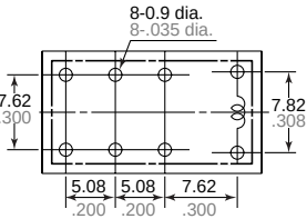
mm inch PC board pattern (Bottom view)
