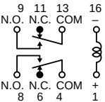
Schematic (Bottom view)
