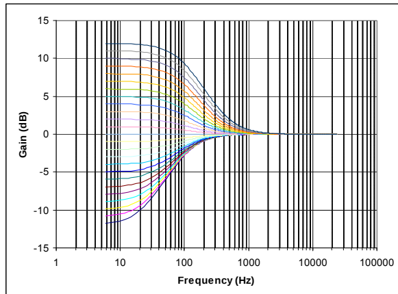
Figure 30 EQ Band 1 – Low Freq Shelf Filter Response
