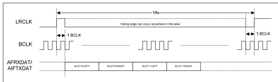
Figure 55 TDM in DSP Mode A
