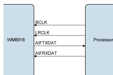
Figure 41 Slave Mode
