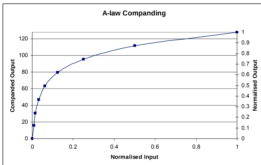
Figure 58 A-Law Companding
