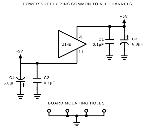
Figure 2: Inverting Op Amp Configuration (Please Follow Page 5 Modification for Inverting Gain)
