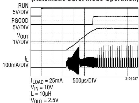
Start-Up from Shutdown (Automatic Burst Mode Operation)
