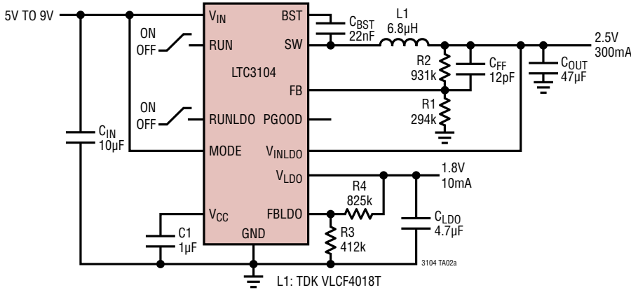
Dual Lithium-Ion to 2.5V/300mA Regulator with 1.8V /10mA LDO
