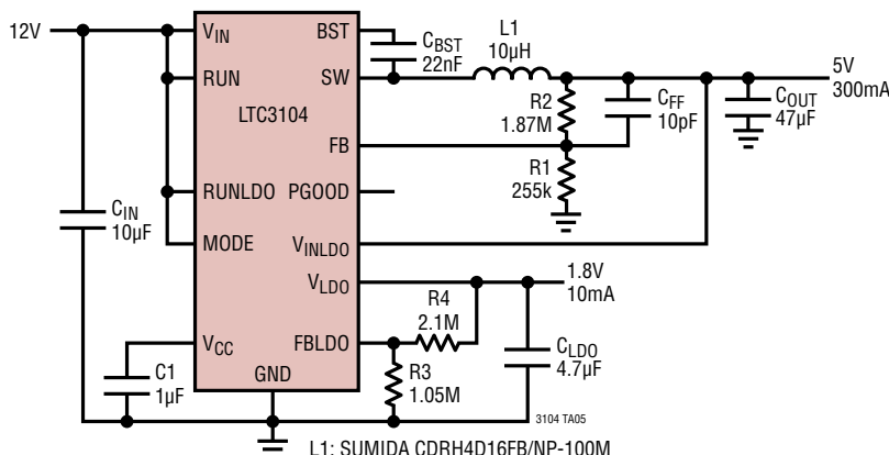
12V to 5V/300mA Regulator with High Efficiency, Ultralow I Q (2.8μA with V OUT in Regulation, No Load) and 1.8V/10mA LDO
