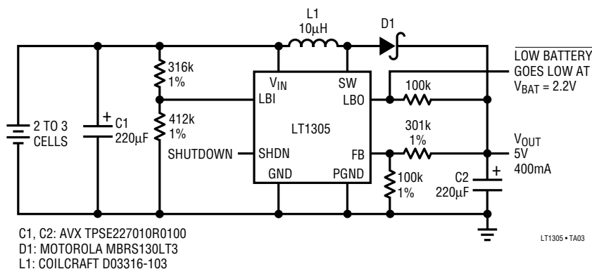
2-Cell and 3-Cell to 5V/400mA DC/DC Converter with Low-Battery Detect
