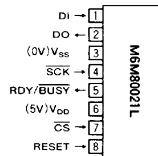
Outline 8P5K
