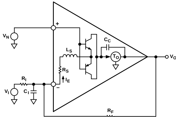
Figure 13. Equivalent Circuit
