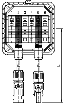
PV-JB/2-2/N... PV-JB/2-2/N...-UR
