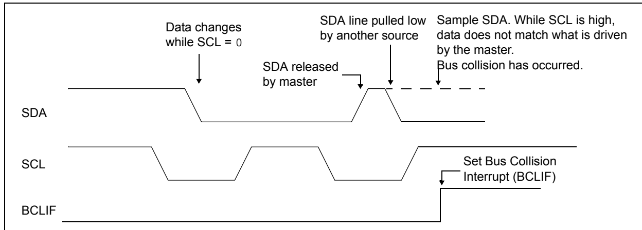
FIGURE 29-24: BUS COLLISION TIMING FOR TRANSMIT AND ACKNOWLEDGE
