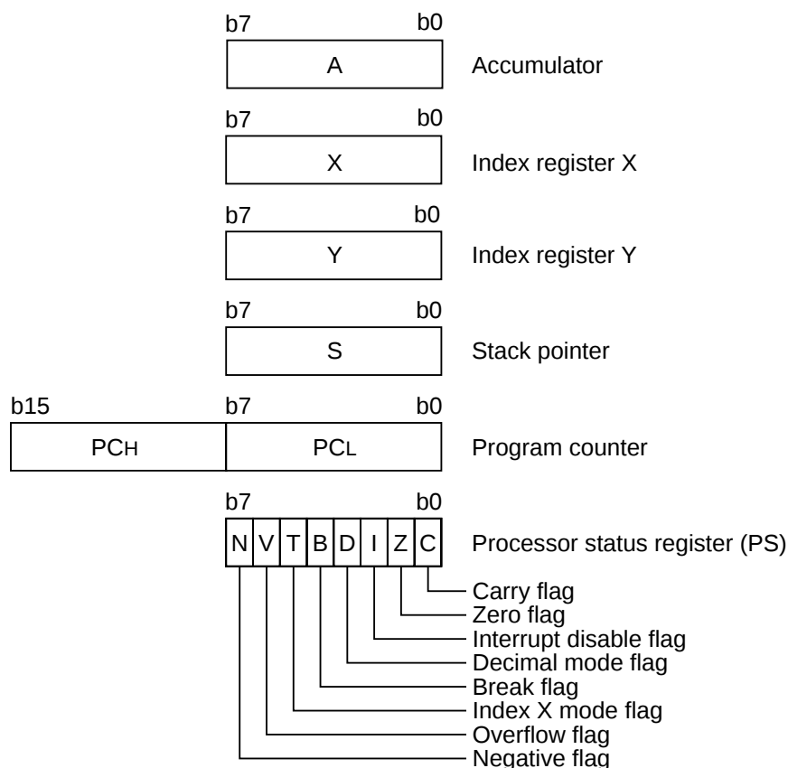
Fig. 7 740 Family CPU register structure
