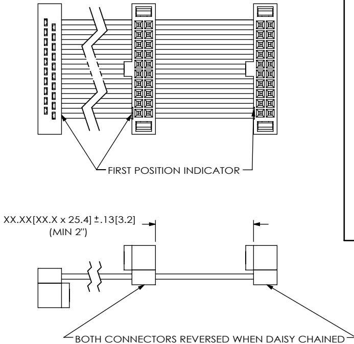
FIG 6 (FFSD-10-D-XX.XX-01-X-N-DXX-R SHOWN) (SAME AS FIG 1, DIFFERENT AS SHOWN) (NOT AVAILABLE WITH -RN1 OR -RN2 OPTION) (2.00[50.8] MINIMUM, 1.00[25.4] INCREMENTS)
