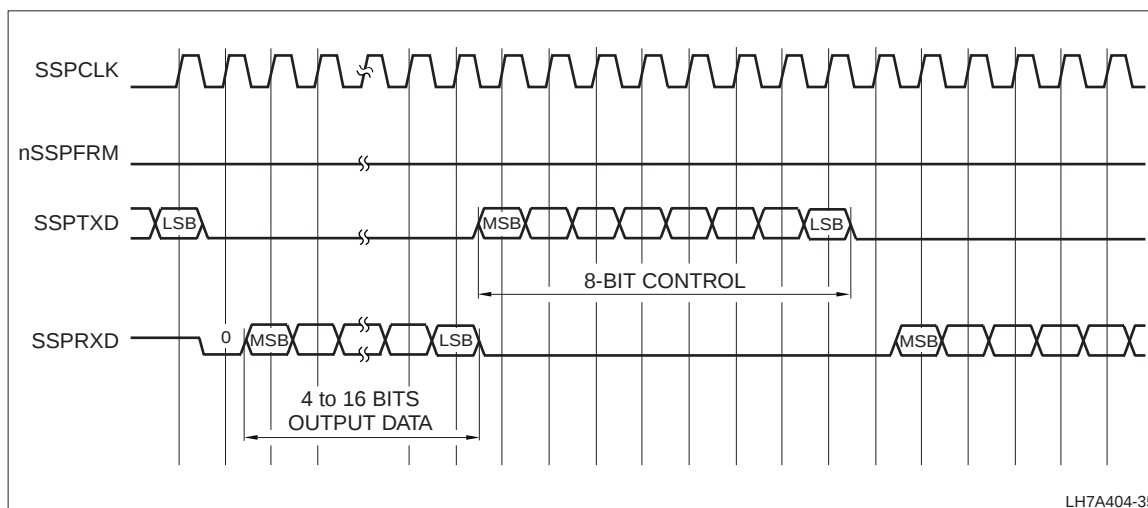
Figure 31. MICROWIRE Frame Format (Continuous Transfers)
