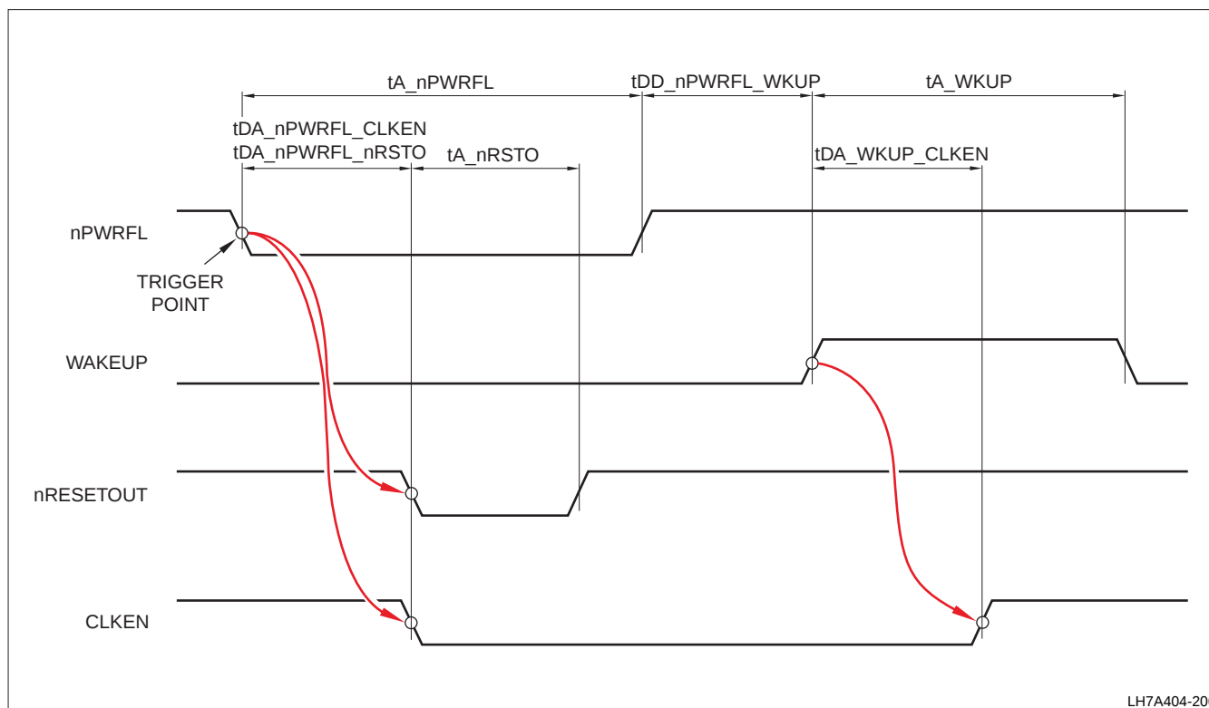
Figure 51. nRESETOUT Timing for nPWRFL Trigger
