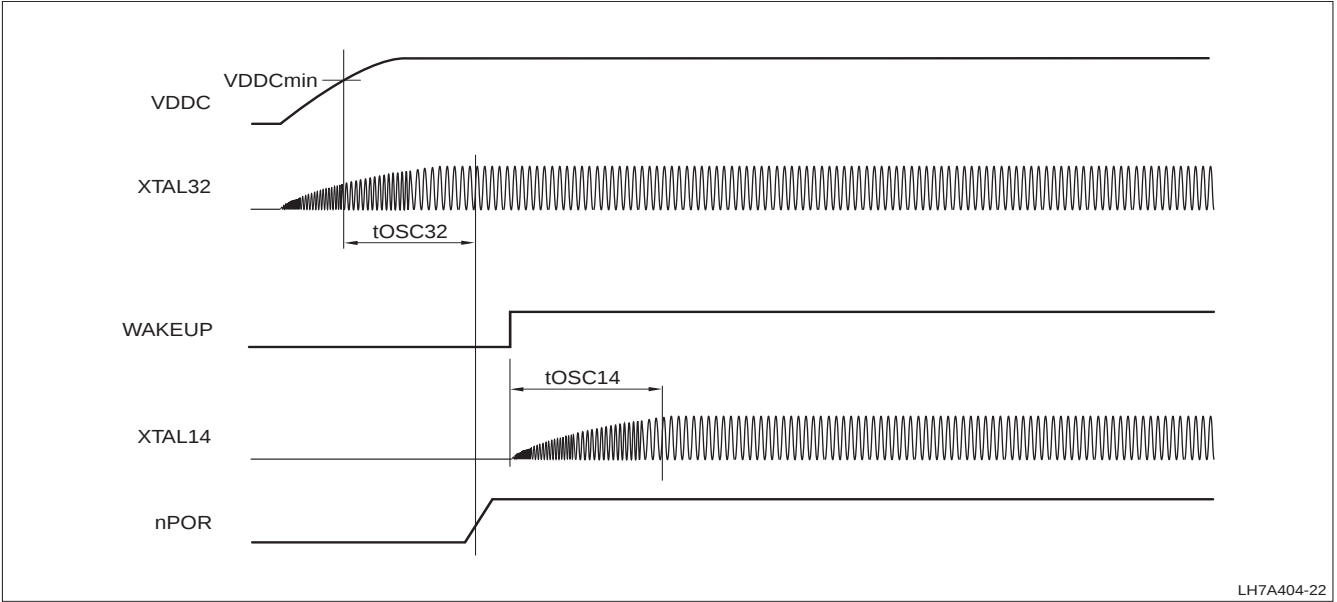
Figure 48. PLL Start-up
