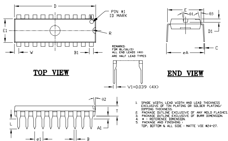
8-Pin Plastic DIP (N)
