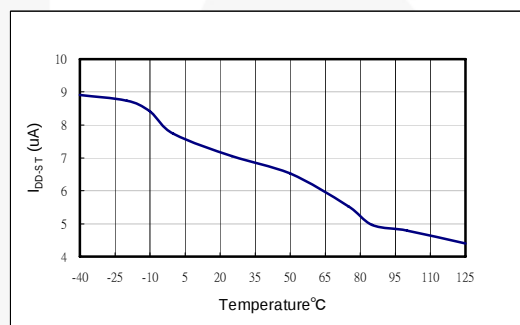
Figure 8. Startup Current
