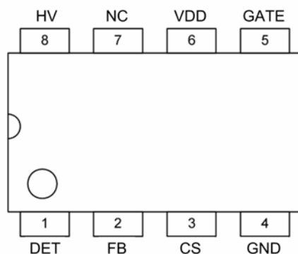
Figure 4. Pin Configuration
