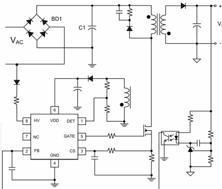
Figure 1. Typical Application
