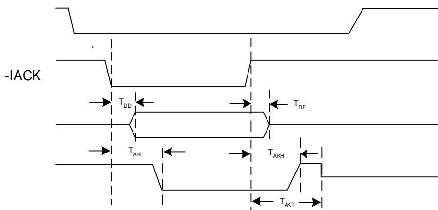
Figure 7: Interrupt Timing
