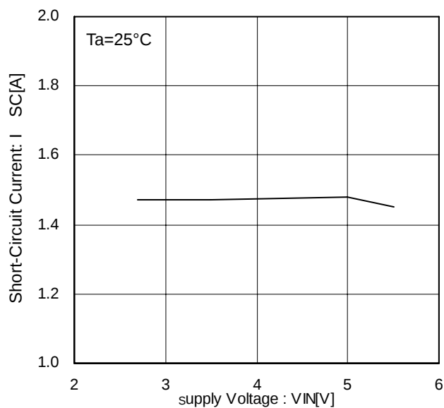
Figure 14. Short circuit current
