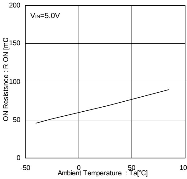
Figure 11. On-resistance
