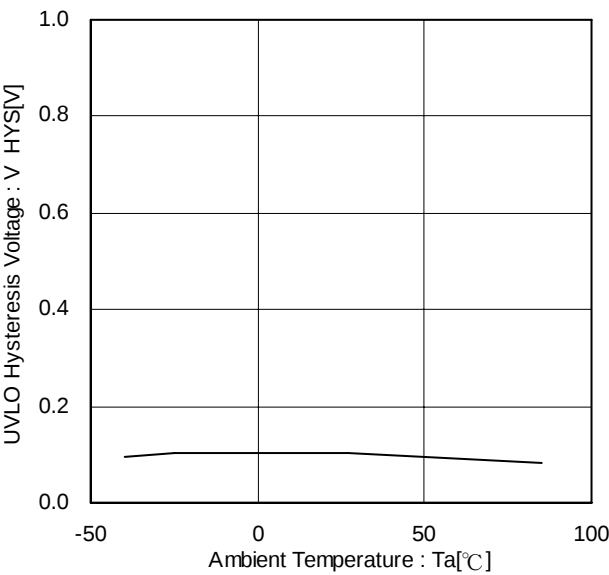
Figure 19. UVLO hysteresis voltage
