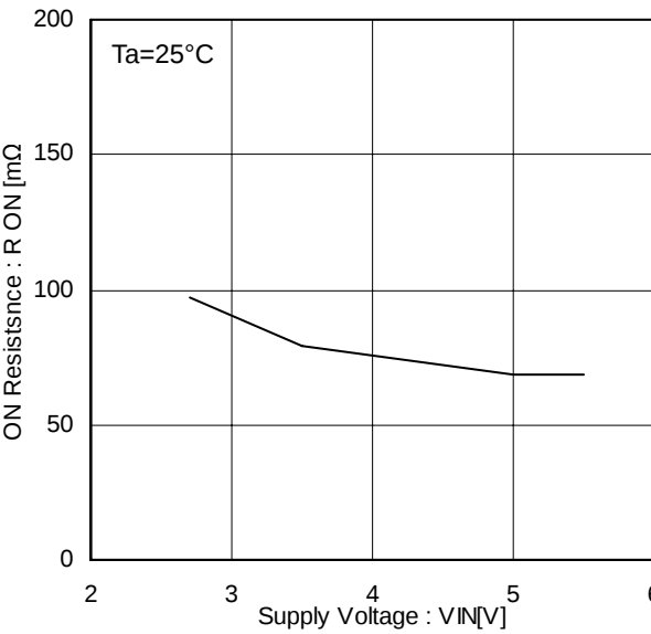
Figure 10. On-resistance
