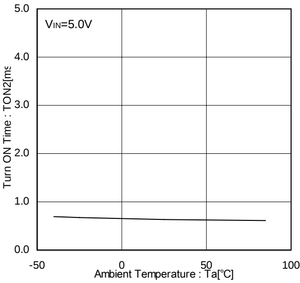
Figure 23. Output turn-on time
