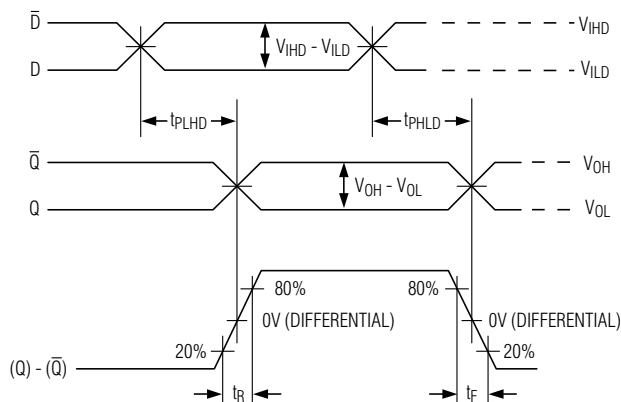
Figure 2. Differential Transition Time and Propagation Delay Timing Diagram
