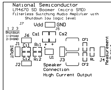
Figure 40. Silk Screen
