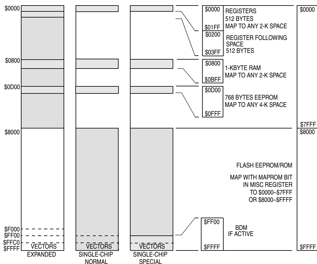
Figure 5-6. Memory Map
