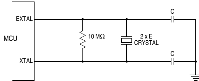
Figure 1-5. Common Crystal Connections
