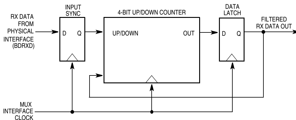
Figure 15-3. BDLC Rx Digital Filter Block Diagram
