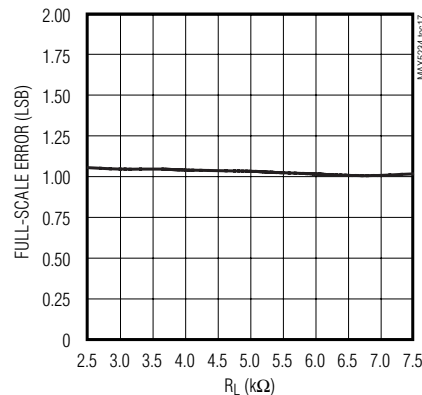
MAX5234 FULL-SCALE ERROR vs. RESISTIVE LOAD
