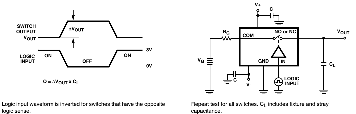
FIGURE 2B. TEST CIRCUIT
