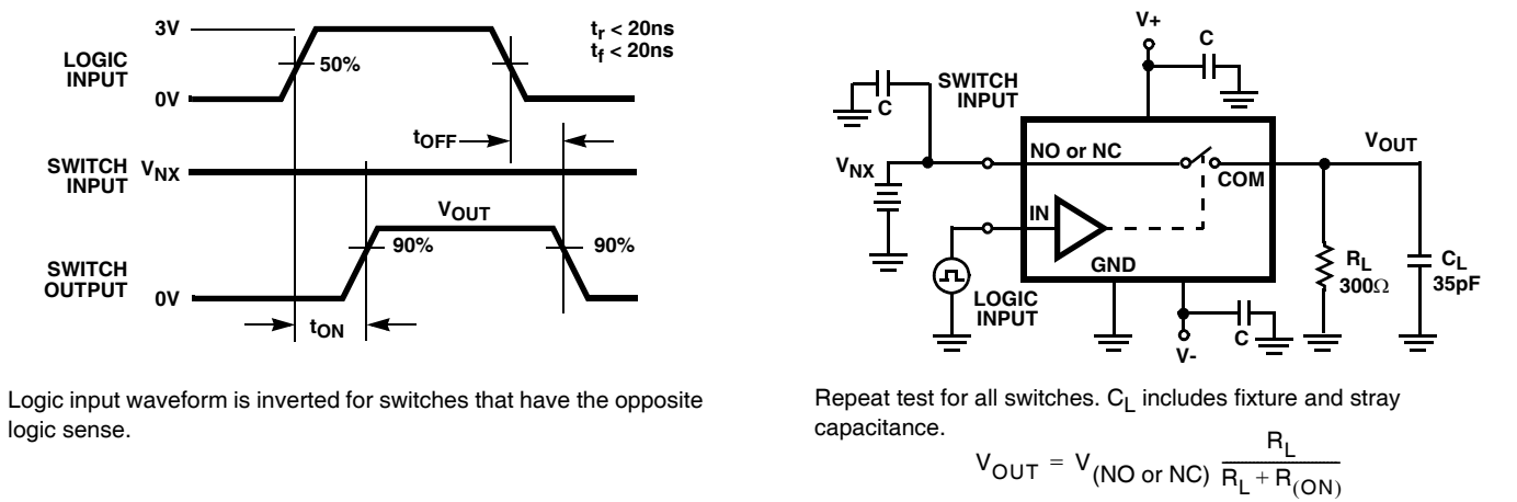
FIGURE 1A. MEASUREMENT POINTS
