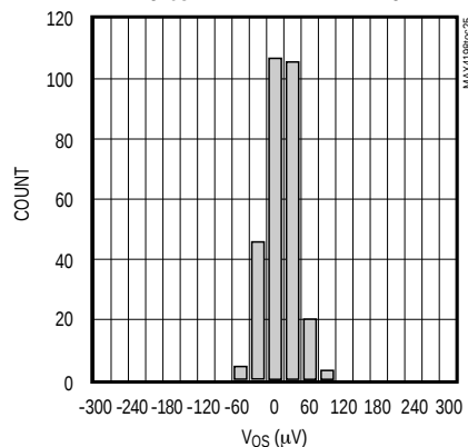
MAX4199 HISTOGRAM ( V_{OS} BASED ON 280 UNITS)
