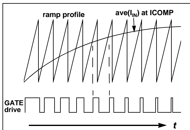
Figure 12 Average Current Control in CCM
