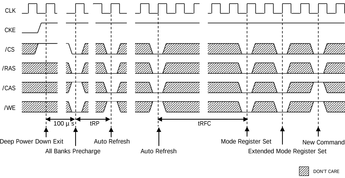
Figure8: Deep Power Down Mode Exit
