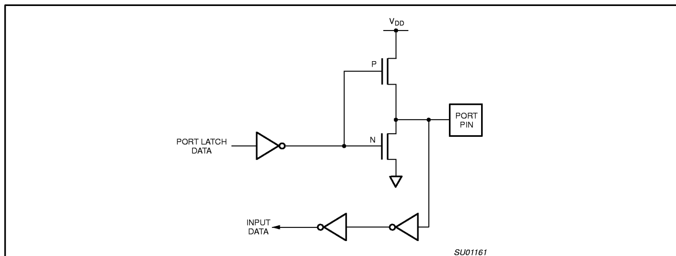
Figure 14. Push-Pull Output
