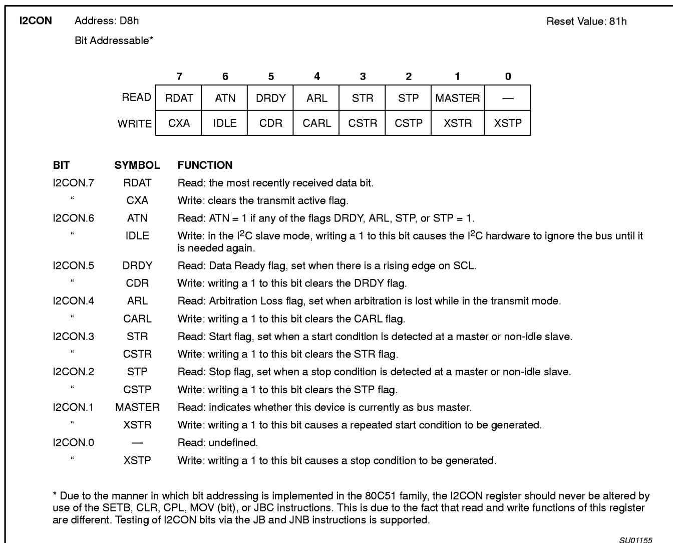
Figure 8. I 2 C Control Register (I2CON)
