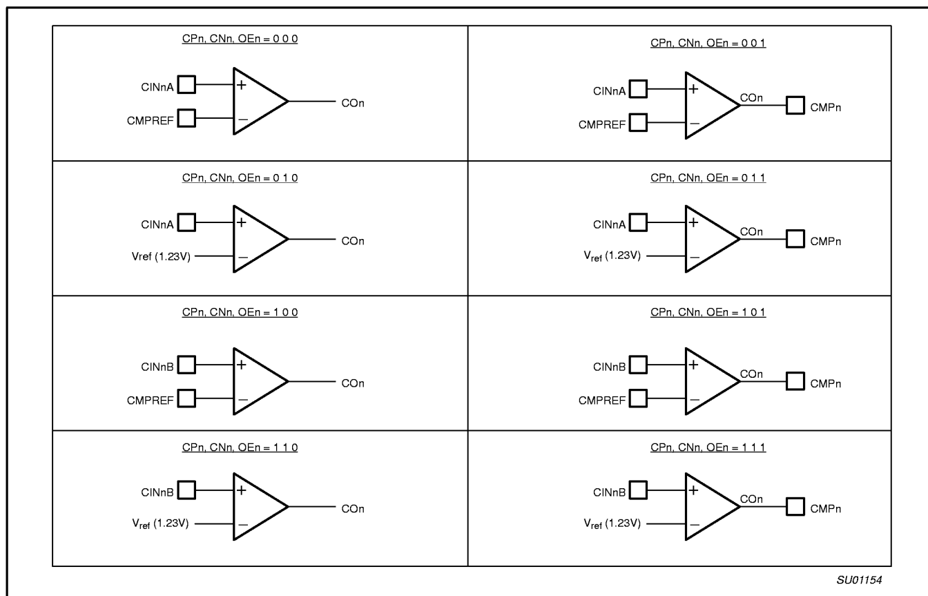
Figure 6. Comparator Configurations
