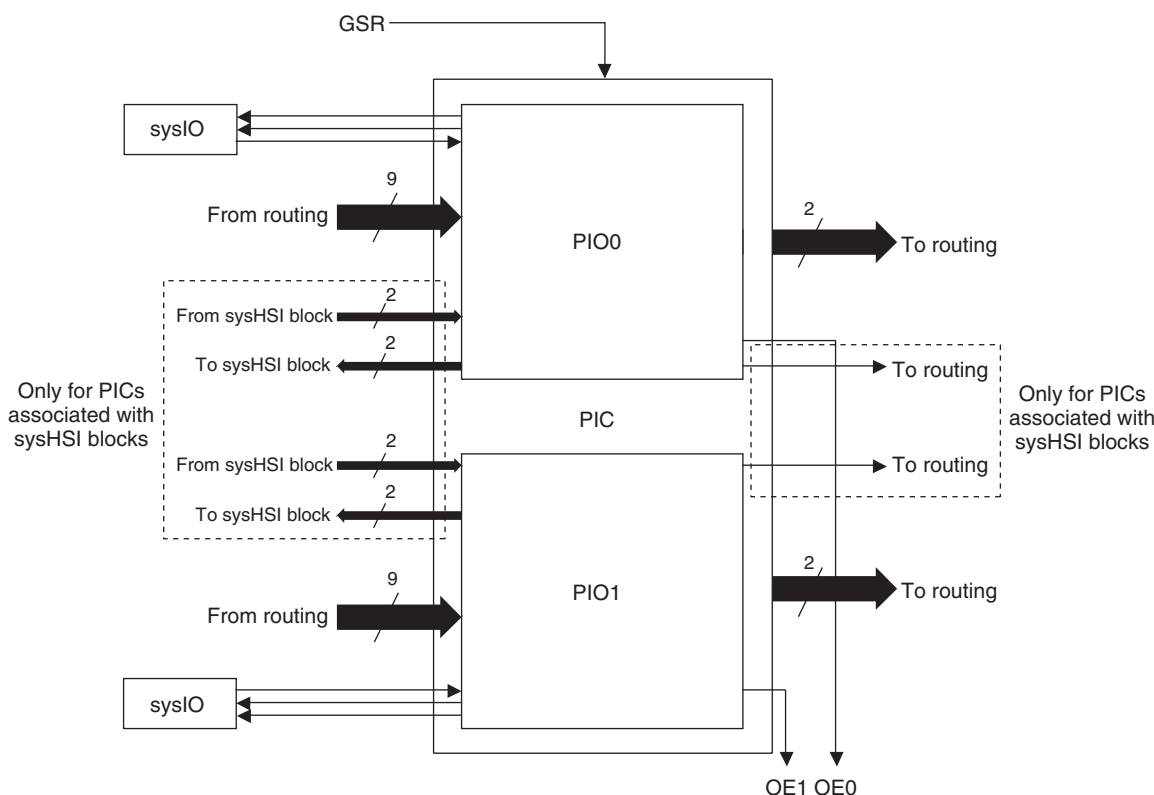
Figure 10. ispXPGA PIC
